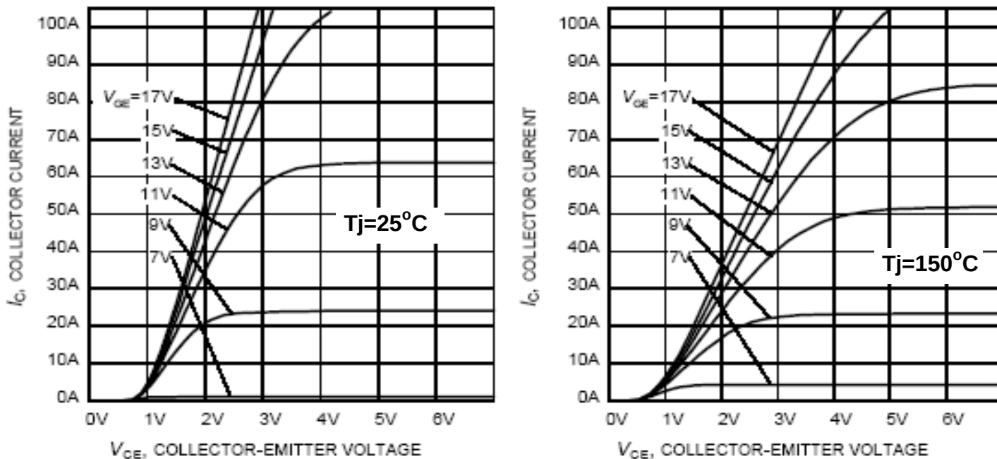
Figure 14. IGBT Conduction Characteristics
