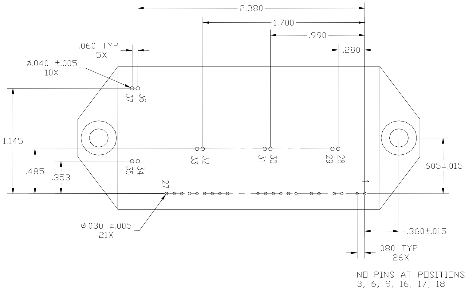
Figure 3 - Package Pin Locations (All dimensions are in inches; tolerance is +/- 0.005" unless otherwise specified)
