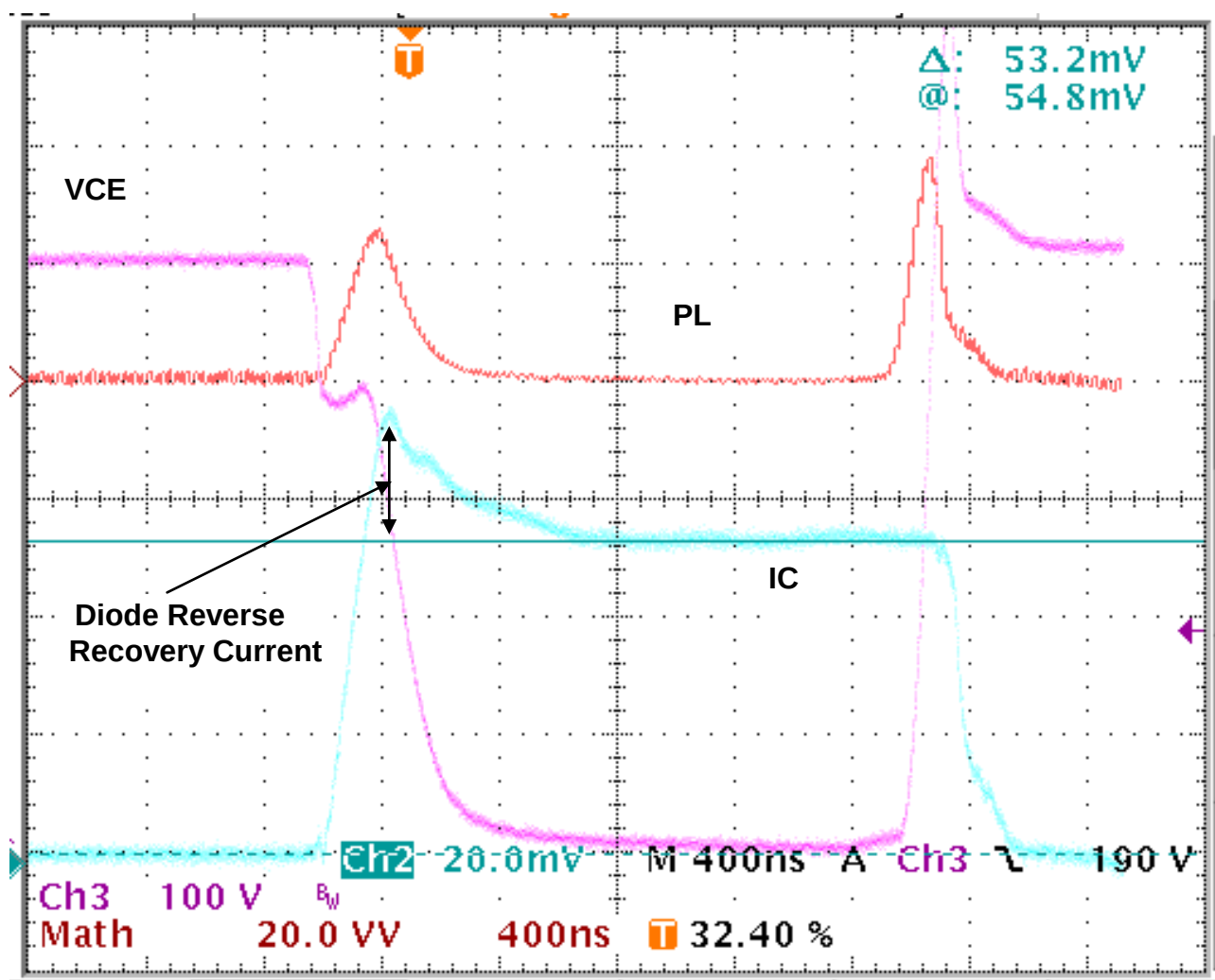
Figure 11. Switching Waveforms at I_C = 53A
