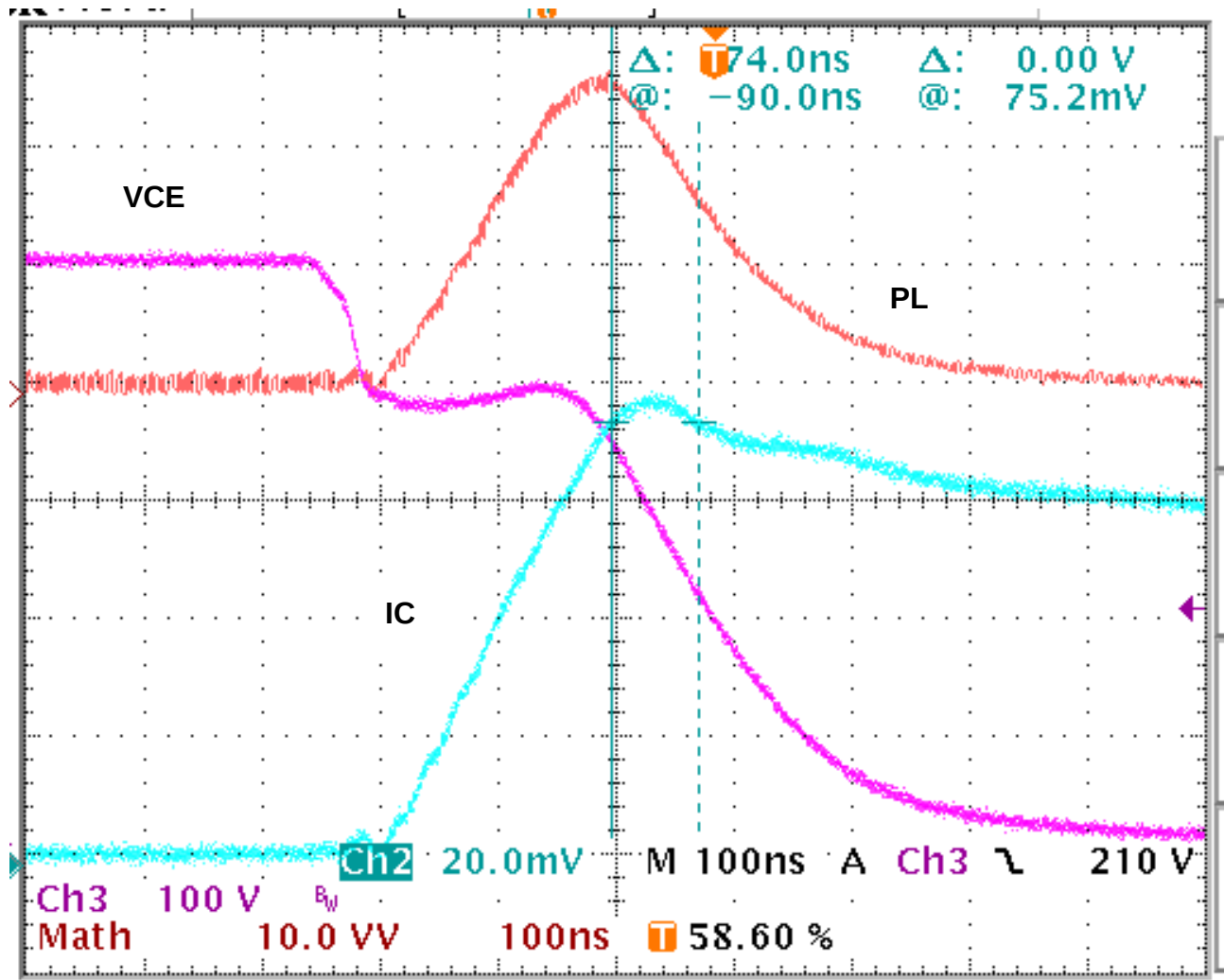
Figure 12. Turn On Switching Waveforms at I_C = 53A
