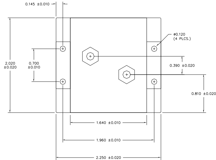
TOP VIEW MECHANICAL LAYOUT DRAWING
